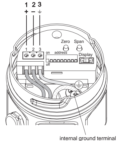
Electrical connection PROFIBUS-PA electronics
