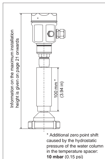
Cerabar M with temperature spacer
