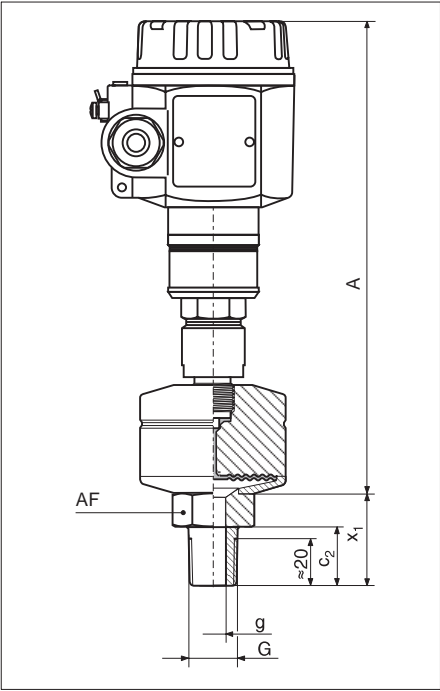
Separator with ½ NPT, ANSI B 1.20.2
