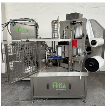
Conditionneuse rotative ATIA type A4003-35 Rotary filling machine
